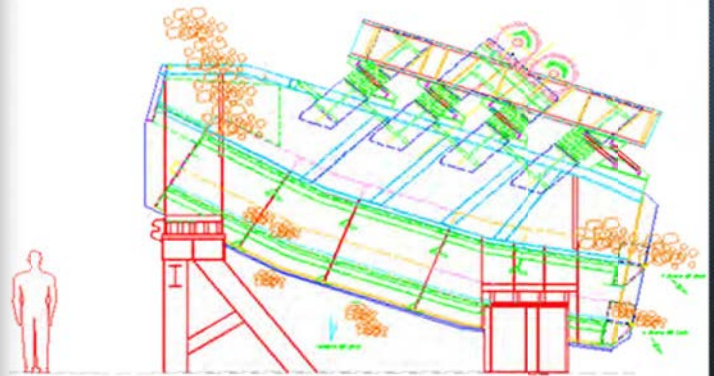
Banana Screen - Typical Arrangement
